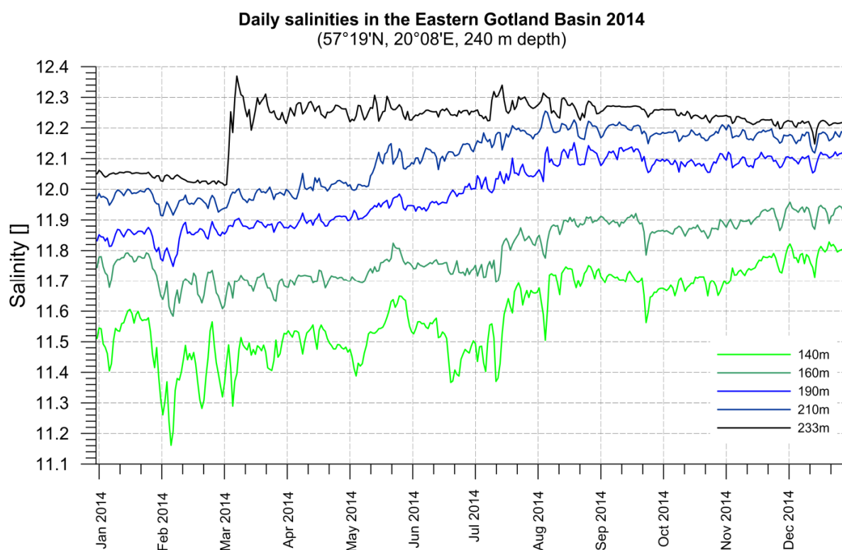
Fig. 28: Temporal development of deep water salinity in the Eastern Gotland Basin (station 271) from January to December 2014 (Daily averages of original data with 10 min sampling interval)
