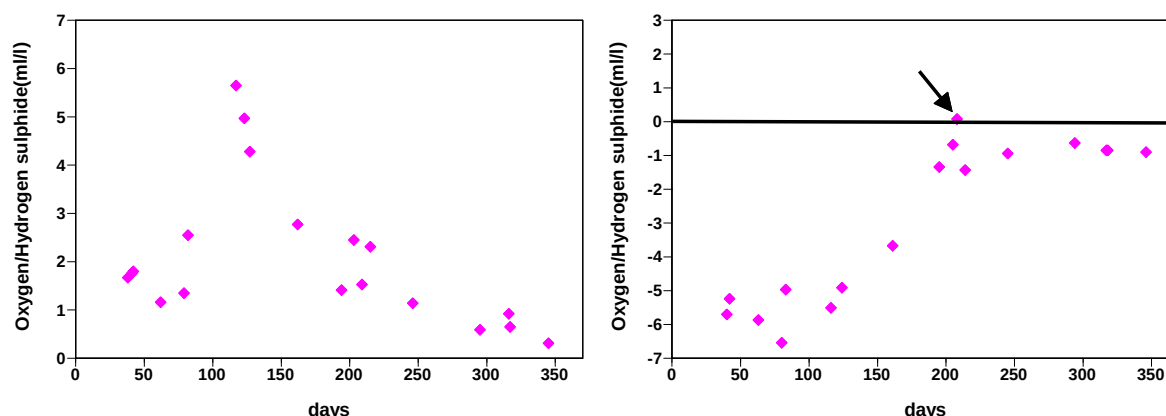
Abb. 36: Development of the oxygen/hydrogen sulphide content in the Bornholm Deep (80 m depth, left) and the eastern Gotland Basin (200 m depth, right) – IOW and SMHI data
