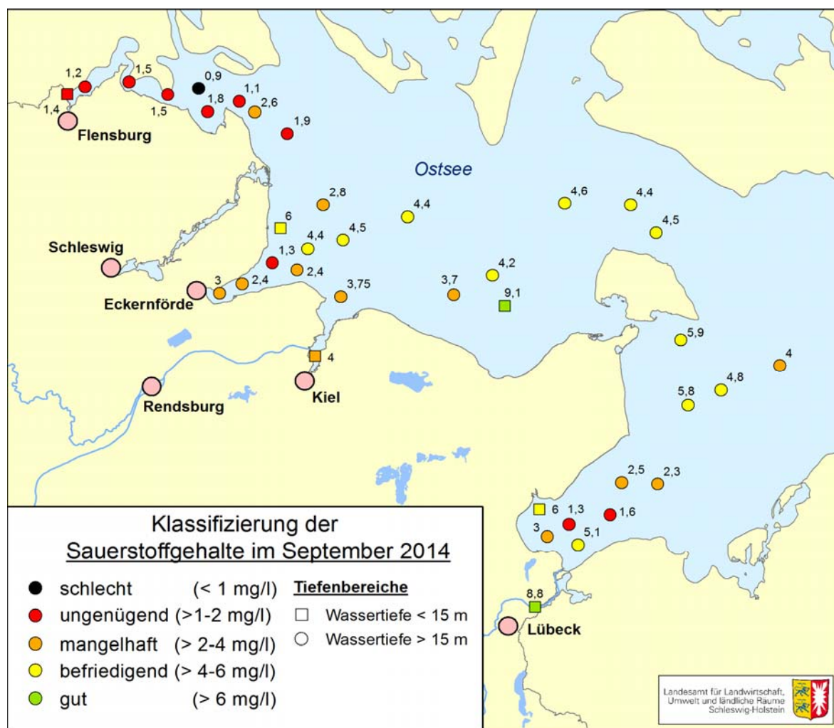
Fig. 32: Oxygen deficiency in the western Baltic Sea in September 2014 (LLUR, 2014) – O_2 \text{ [mg/l]} \times 0.7005 = O_2 \text{ [ml/l]}
