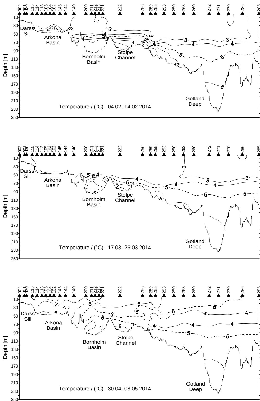
Fig. 25: Vertical water temperature distribution 2014 between Darss Sill and northern Gotland Basin
