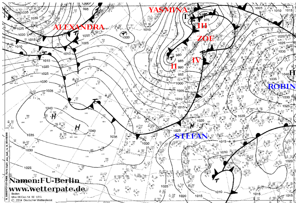
Fig. 3: Weather chart of 8 December 2014 with a storm front over the North Atlantic (FU-Berlin, 2014)
