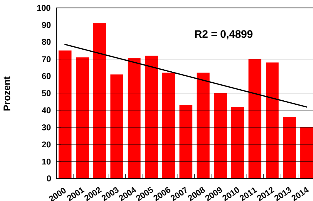
Fig. 34: Percentage of stations with an oxygen content < 2mg/l in the bottom near layer in the western Baltic Sea in autumn – data LLUR
