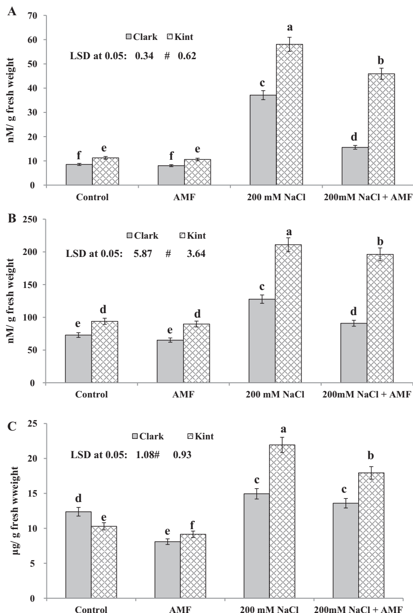
Fig. 2 (A–C) Thiobarbituric acid reactive substances (TBARS) (A), H_2O_2 (B) and malondialdehyde (MDA) (C) in soybean ( Glycine max L. Merr) genotypes with different salt stress tolerance inoculated with AMF under salt stress. Columns represent the means for five plants ( N = 5 ) with error bars showing standard deviation. Values denoted by different letters are significantly different at P < 0.05 .
