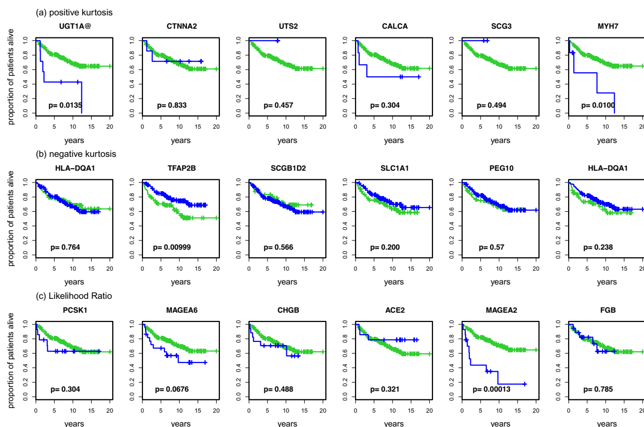
Figure 7 Kaplan-Meier curves for the top 6 genes for positive and negative Kurtosis and the likelihood ratio. Kaplan-Meier curves for the top 6 detected genes for positive and negative Kurtosis and the likelihood ratio. In every graphic the green line denotes the survival in the group with lower expression values for the corresponding gene and the blue line the survival in the group with higher expression values. The graphics also contain the corresponding p-values of the logrank test.
