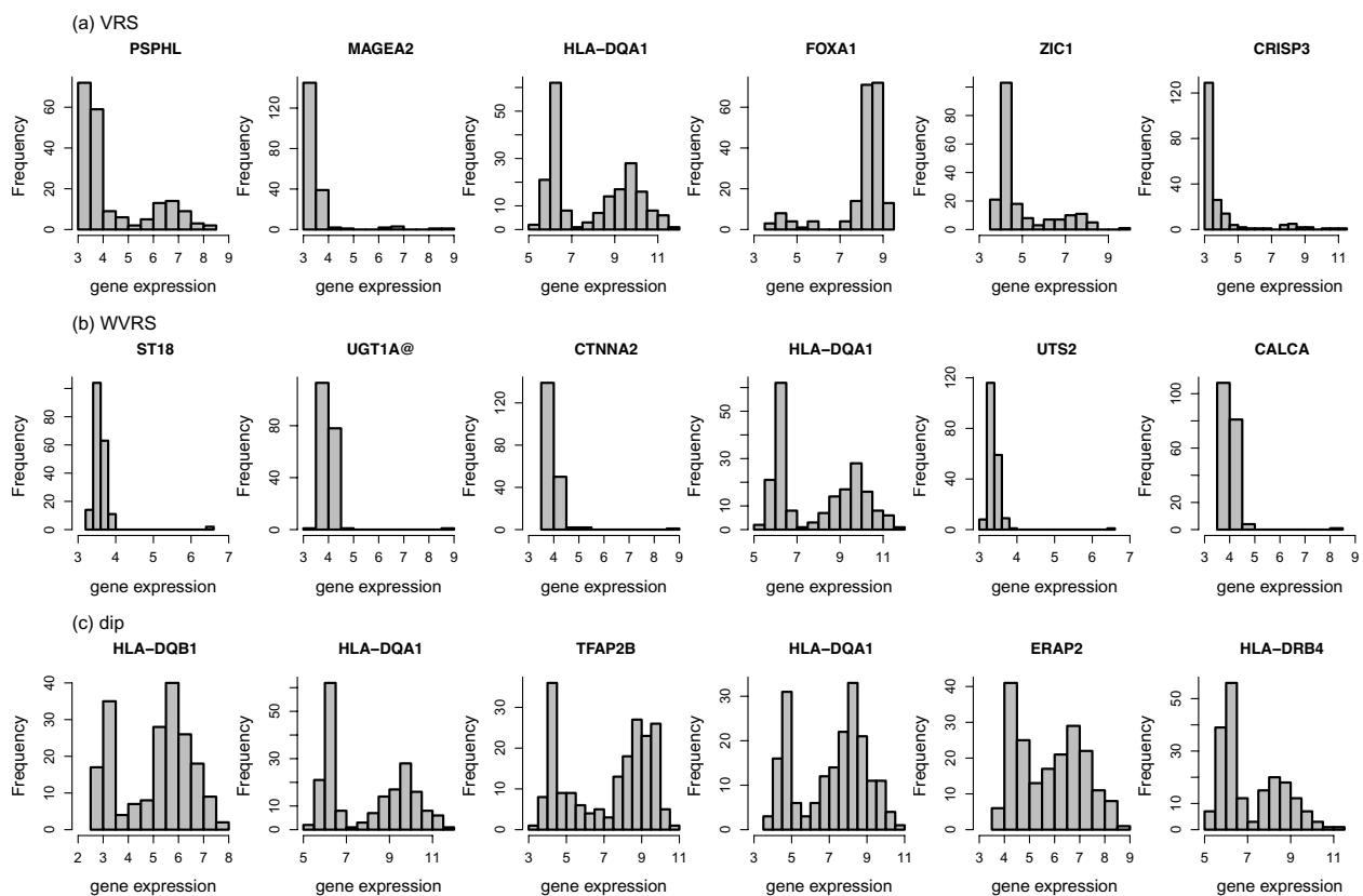
Figure 3 Histograms of the top 6 genes for WVRs, VRS and dip.
