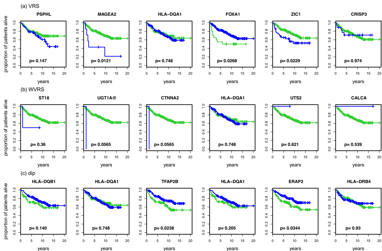
Figure 6 Kaplan-Meier curves for top 6 genes for WVRs, VRS and dip. Kaplan-Meier curves for the top 6 detected genes for WVRs, VRS and dip. In every graphic the green line denotes the survival in the group with lower expression values for the corresponding gene and the blue line the survival in the group with higher expression values. The graphics also contain the corresponding p-values of the logrank test.
