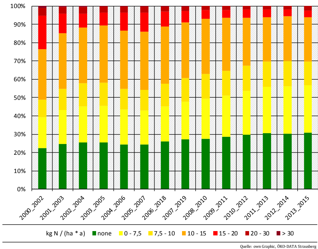
Abbildung 10: Exceedance of Critical Load for Eutrophication in the years 2000 to 2015 averaged over three years of nitrogen input rates
