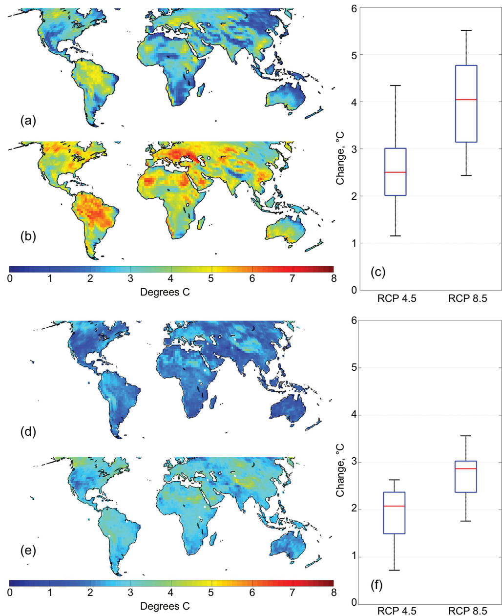
Figure 1. Panels (a)–(c): changes in annual maximum air temperature in 2060–2080 relative to 1985–2005 under RCP 4.5 (a) and RCP 8.5 (b). Panel (c) shows the range in projected annual maximum temperature increase spatially averaged over land for both emission scenarios over all 18 CMIP5 GCMs. Panels (d)–(f): same as (a)–(c) except for annual maximum wet bulb temperature. Air temperatures increase at a faster rate and have more spatial variability than wet bulb temperatures, in part due to the dependence of wet bulb temperature on humidity.
