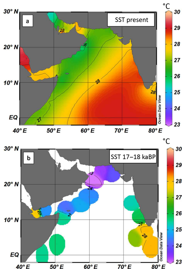
Figure 4. Annual SST distribution in ^{\circ}\text{C} from the World Ocean Atlas (Locarnini et al., 2013) (a); alkenone- and Mg/Ca-derived SST reconstruction for the time slice from 17–18 ka BP (b) from cores shown in Fig. 1.
