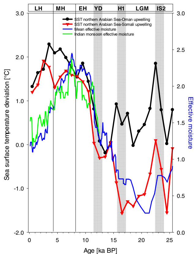
Figure 7. Millennial regional-averaged SST from the northern Arabian Sea minus Oman-upwelling-averaged SST in °C (black line) and northern Arabian Sea minus Somali-upwelling-averaged SST (red line; regions are indicated in Fig. 1) compared with reconstructions of the mean effective moisture in southern and central Asia (blue line) and the Indian monsoon region (green line) from continental archives (Herzschuh, 2006). Grey bars and abbreviations as in Fig. 3.
