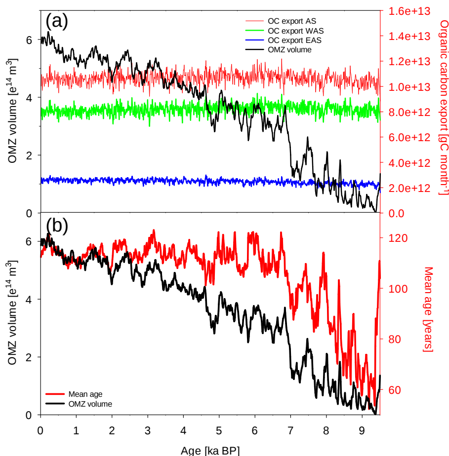
Figure 8. Simulated volume of the Arabian Sea OMZ ( 70 \mu\text{mol L}^{-1} threshold, black) and export production in the entire Arabian Sea (red), western Arabian Sea (green) and eastern Arabian Sea (blue) over the Holocene (a). OMZ volume and age of water masses (time since contact with the surface) averaged over the OMZ (b). Arabian Sea defined as 55\text{--}75^\circ \text{E} , 8.5\text{--}22.5^\circ \text{N} ; border between west and east defined at 68.5^\circ \text{E} .
