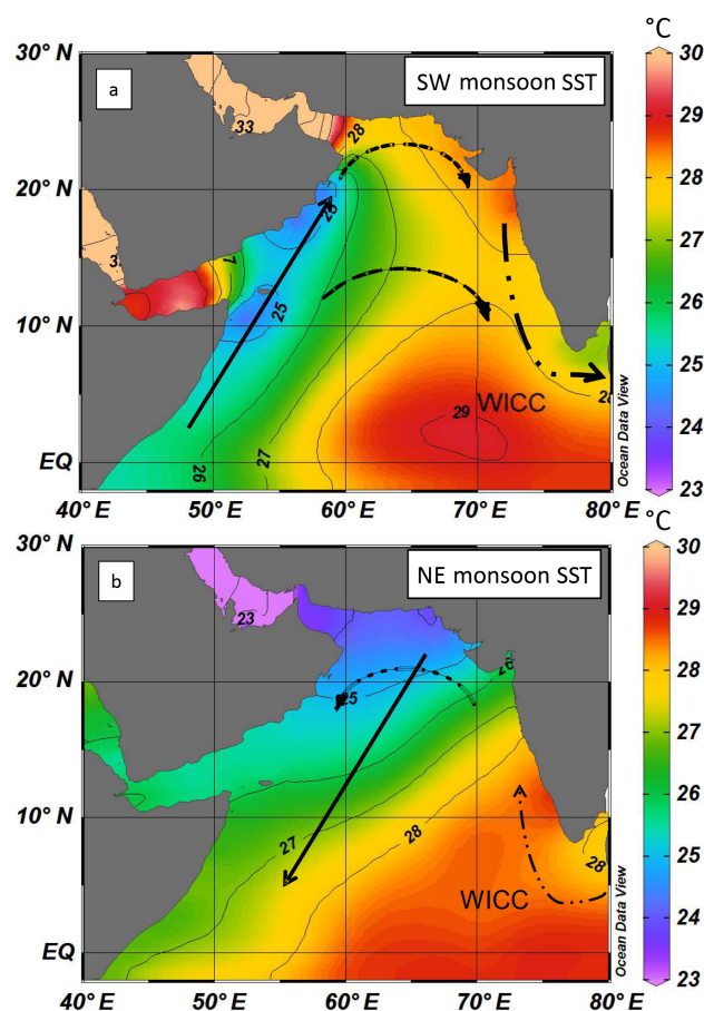
Figure 2. SST in ^{\circ}\text{C} from Jul–Sep (SW monsoon) (a) and Jan–Mar (NE monsoon) (b) from the World Ocean Atlas (Locarnini et al., 2013). Solid arrows indicate major wind directions and broken arrows indicate surface general currents; WICC is the West Indian Coastal Current.
