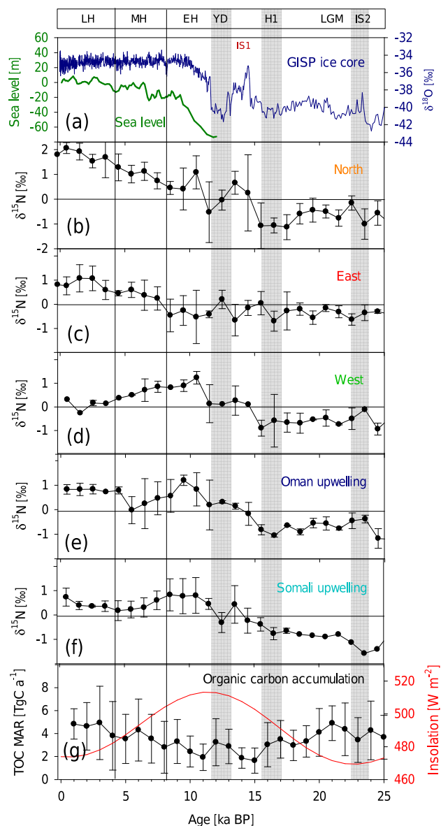
Figure 6. The \delta^{18}\text{O} values in ‰ from the GISP2 ice core (Groote and Stuiver, 1997) and sea level (m above NN) reconstruction from the Red Sea (Siddall et al., 2003) (a) compared with millennial regional averages of normalized and averaged \delta^{15}\text{N} (‰) values from the northern (b), eastern (c), and western (d) Arabian Sea, the Oman (e), and Somali (f) upwelling area. Total organic carbon mass accumulation in the Arabian Sea (TOC MAR in \text{Tg C year}^{-1} ; data from Cartapanis et al., 2016, and Tim Rixen, unpublished) and insolation at 30^\circ\text{N} in \text{W m}^{-2} (Berger and Loutre, 1991) (g) during the last 25 kyr. Error bars denote \pm 1\sigma . Grey bars and abbreviations as in Fig. 3; interstadial 1 (IS1).
