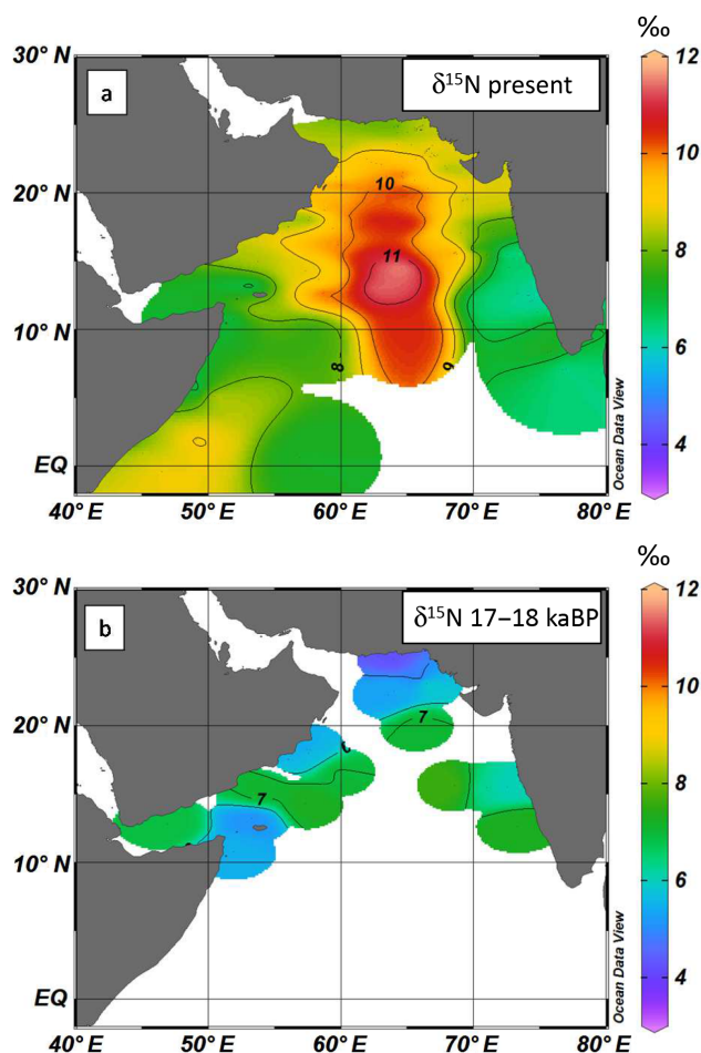
Figure 5. The \delta^{15}\text{N} values in ‰ in recent surface sediments (a); \delta^{15}\text{N} in sediments at 17–18 ka BP (b) from surface and core locations shown in Fig. 1.
