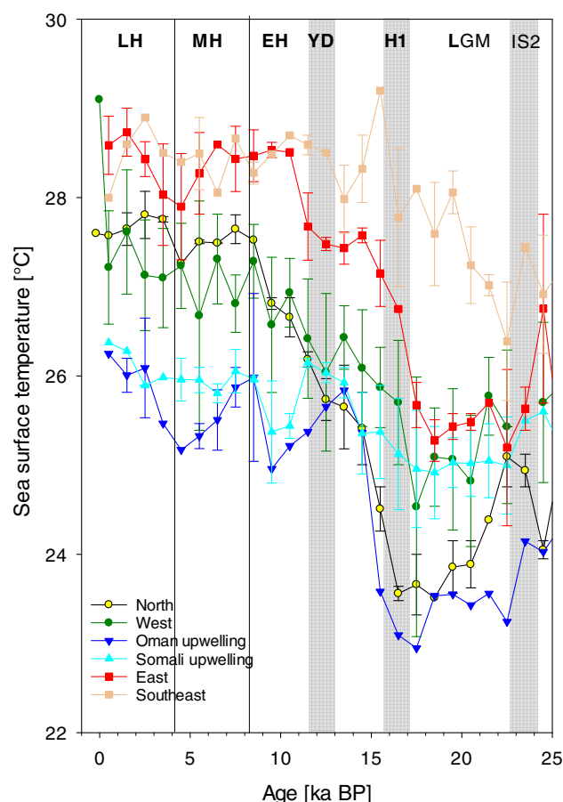
Figure 3. Millennial regional averages of SST ( ^{\circ}\text{C} ) and \pm 1\sigma standard deviation in the northern, western, eastern, and southeastern Arabian Sea and the Oman and Somali upwelling areas of the last 25 kyr. Regions are indicated in Fig. 1. Times of interstadial 2 (IS2), Heinrich Event 1 (H1), and Younger Dryas (YD) are indicated by grey bars. The last glacial maximum (LGM), early Holocene (EH), mid-Holocene (MH), and late Holocene (LH) are also marked. Lines mark the beginning of MH and LH.
