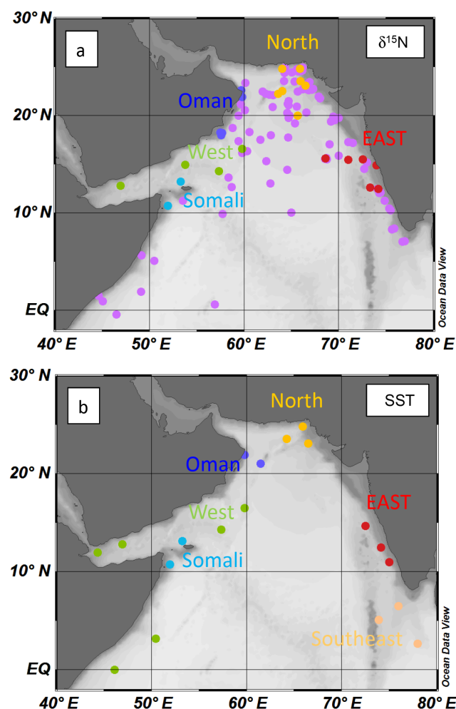
Figure 1. Stations of sediment cores for \delta^{15}\text{N} (a) and for SST (b) reconstructions with colors indicating surface sediment samples (purple) and cores from the Oman upwelling (dark blue), Somali upwelling (light blue), and the western (green), northern (yellow), eastern (red), and southeastern (orange) Arabian Sea.
