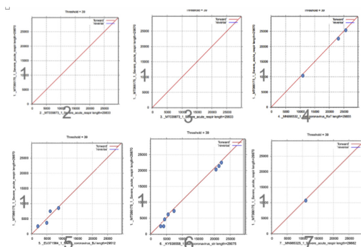
FIG. 2. MAFFT considers similarities in forward strands (red) only, but ignores similarities in reverse strands (blue), Plot 1/2: alignment MT066175.1 + MT039873.1 99.7%, plot 1/3: MT066175.1 + MN997409.1 99.7%, plot 1/4: MT066175.1 + MN996532.1 89%, plot 1/5: MT066175.1 + EU371564.1 82.4%, plot 1/6: MT066175.1 + KY938558.1 = 68%, plot 1/7: MT066175.1 + MN985325.1 95%.
