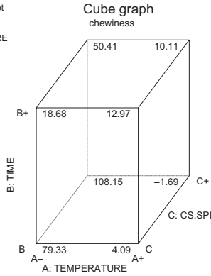
DESIGN-EXPERT Plot Chewiness X = A: TEMPERATURE Y = B: TIME Z = C: CS:SPI
