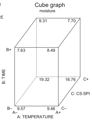
DESIGN-EXPERT Plot moisture X = A: TEMPERATURE Y = B: TIME Z = C: CS:SPI
