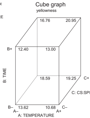
DESIGN-EXPERT Plot yellowness X = A: TEMPERATURE Y = B: TIME Z = C: CS:SPI
