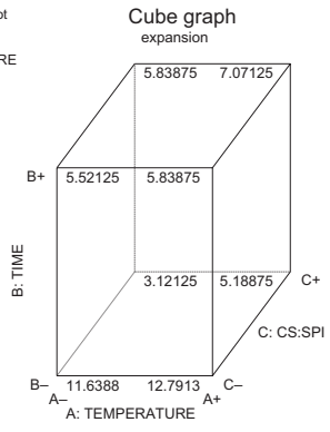
DESIGN-EXPERT Plot expansion X = A: TEMPERATURE Y = B: TIME Z = C: CS:SPI
