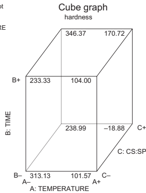
DESIGN-EXPERT Plot hardness X = A: TEMPERATURE Y = B: TIME Z = C: CS:SPI
