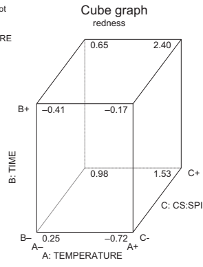
DESIGN-EXPERT Plot redness X = A: TEMPERATURE Y = B: TIME Z = C: CS:SPI
