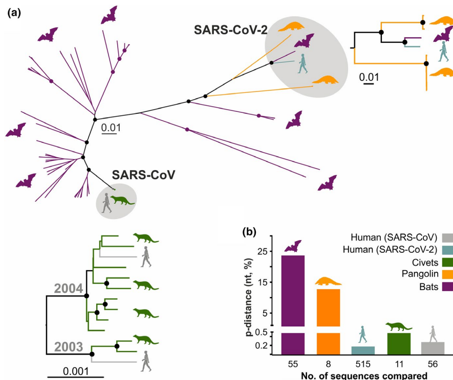
FIGURE 2 Mammalian hosts of coronaviruses. (a) Large diversity of bat-associated SARS-related CoVs in comparison to other hosts. The phylogeny was constructed with 77 SARS-related CoV full-length genomes using a neighbour-joining method with 1,000 bootstrap replicates. Circles at nodes indicate bootstrap values \geq 75\% . Scale bar indicates nucleotide substitutions per site. (b) High divergence of bat SARS-related CoVs in comparison with viruses infecting pangolin, civet and human hosts. P-distance within SARS-related CoVs in each host. The human SARS-CoV-2 and SARS-CoV genomes included all sequences found in GenBank as of 16.04.2020, excluding identical genomes. GenBank accession numbers of all other genomes used in panel A and B: Bat SARS-related CoVs: MN996532, MG772934, MG772933, KY938558, KU182964, KJ473811, KY770860, KJ473813, KJ473812, DQ412042, KY770859, KY770858, BKJ473816, KY417145, KF294455, DQ071615, KY417152, KY417151, KF367457, KC881006, KC881005, KY417144, KY417150, KT444582, KY417146, KY417149, KY417143, FJ588686, KY417148, KY417147, KP886809, KP886808, KJ473815, KU973692, KF569996, KJ473814, DQ648857, DQ412043, JX993987, KF294457, GQ153548, GQ153546, GQ153545, GQ153544, GQ153541, GQ153539, GQ153540, DQ084199, DQ084200, DQ022305, GQ153547, GQ153543, GQ153542, KY352407, GU190215; Human SARS-CoV-2: MN908947; Human SARS-CoV: AY568539, AY390556; Civet SARS-CoV: AY572034, AY572035, AY686863, AY686864, AY304486, AY304488, AY572038, AY686864, AY613948, AY613949, AY613950; and Pangolin SARS-related CoVs: MT121216, MT040335, MT072865, MT072864, MT040336, MT040334, MT040333
