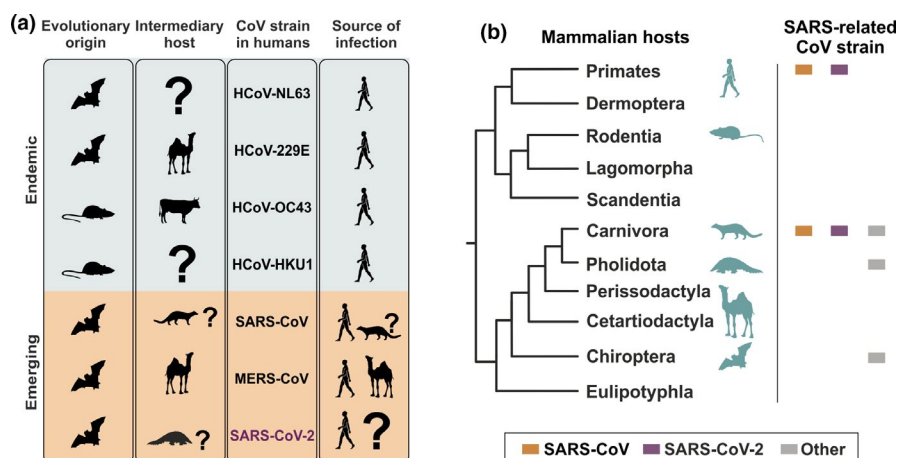
FIGURE 1 Mammals as reservoirs and intermediary hosts of endemic and emerging human coronaviruses. (a) Animal reservoirs and intermediary hosts of human coronaviruses. (b) Cladogram of mammalian orders adapted from (Foley et al., 2016). Hosts of coronaviruses are depicted by pictograms (teal). Squares depict families susceptible to SARS-CoV (orange), SARS-CoV-2 (purple) and other SARS-related CoVs (grey)
