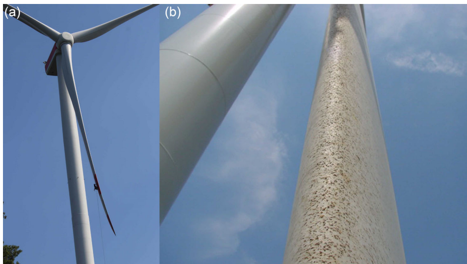
FIGURE 1 Wind turbine with a blade-cleaning maintenance worker (a). Insect detritus at the leading edge of blades (b) (Jose Luis Ruiz, Bladecleaning S.A.)
