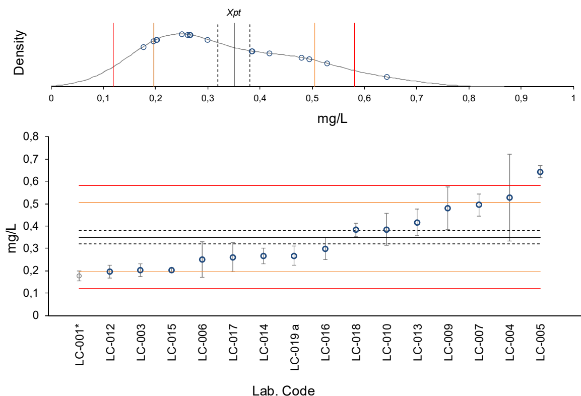
Figure 3: Measurement result range reported by the participants for the determination of Al in cold water extracts of sample 1. Circles and bars represent the reported results [x_i] with the corresponding expanded uncertainties [U(x_i)] ; orange and red lines represent z scores = 2 and 3, respectively; solid and dotted black lines represent the assigned value [x_{pt}] and its expanded uncertainty [U(x_{pt})] .
