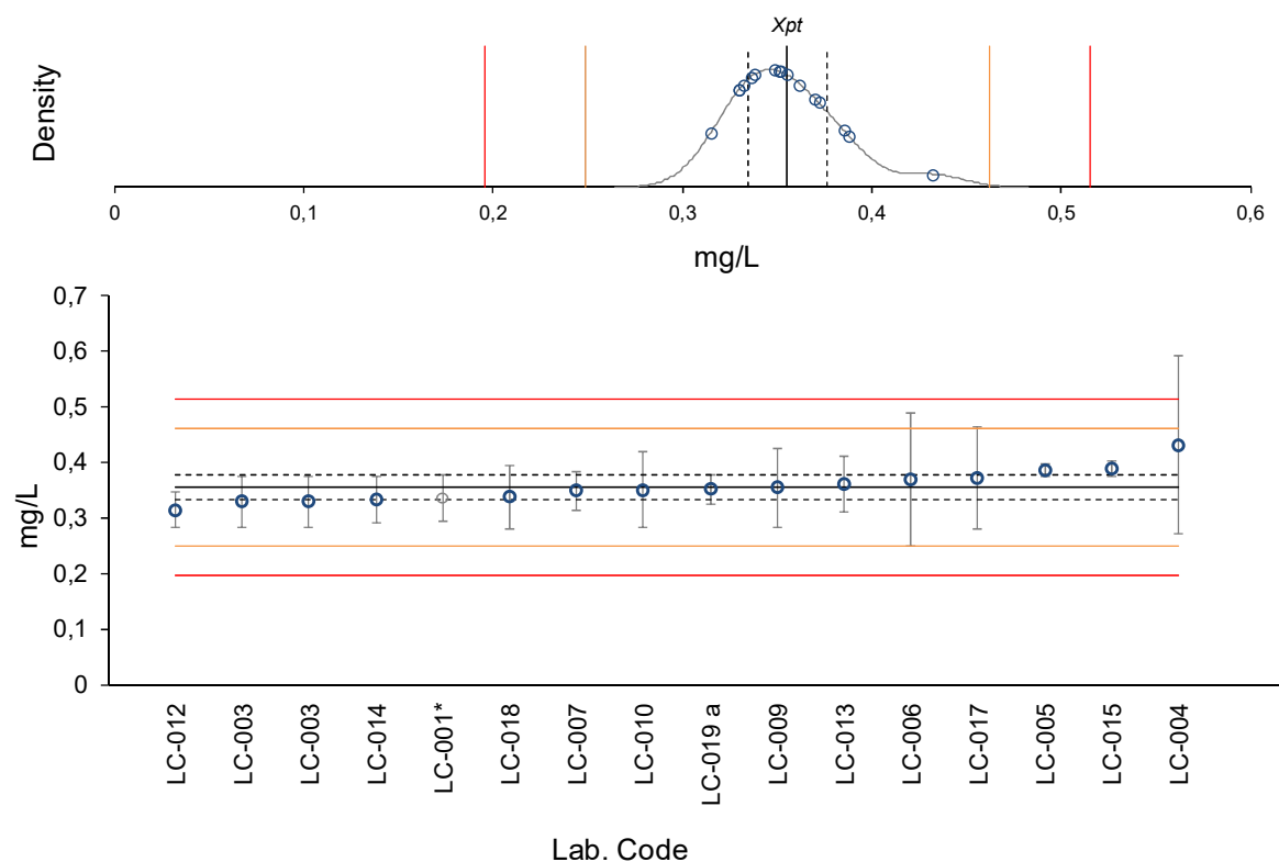
Figure 4: Measurement result range reported by the participants for the determination of Al in solution 3. Circles and bars represent the reported results [x_i] with the corresponding expanded uncertainties [U(x_i)] ; orange and red lines represent z scores = 2 and 3, respectively; solid and dotted black lines represent the assigned value [x_{pt}] and its expanded uncertainty [U(x_{pt})] .
