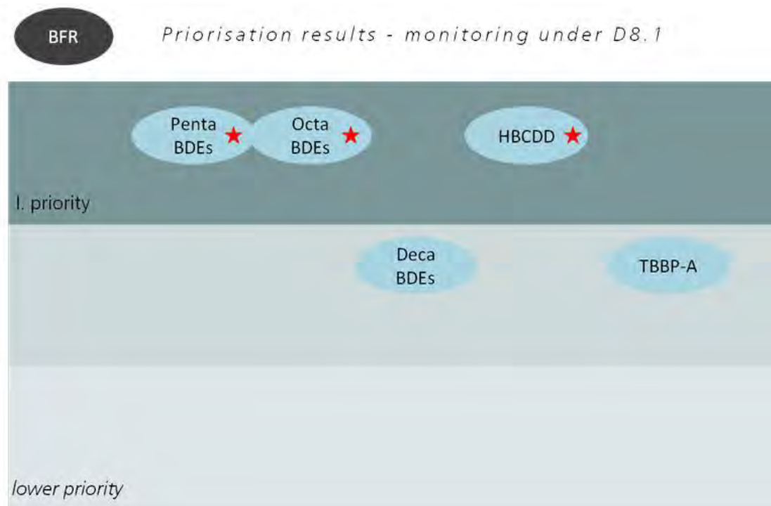
Figure 5-21: Substances proposed for monitoring under D8 – “BFR”.
