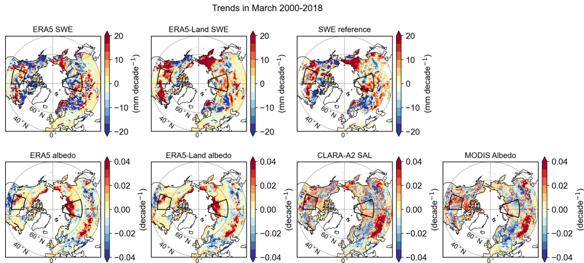
Figure 10. (Top row) SWE trends in March 2000–2018, (bottom row) albedo trends in March 2000–2018.
