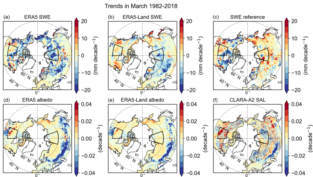
Figure 9. (a, b, c) SWE trends in March 1982–2018. (d, e, f) Albedo trends in March 1982–2018.
