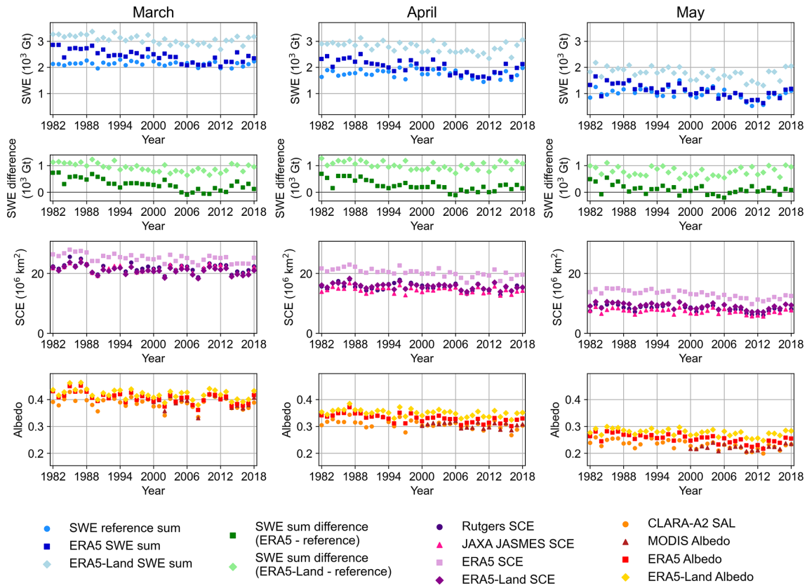
Figure 6. Time series in Eurasia in (left) March, (middle) April, and (right) May for SWE sum (top row), the difference in SWE sum (second row), SCE (third row), and albedo (bottom row).
