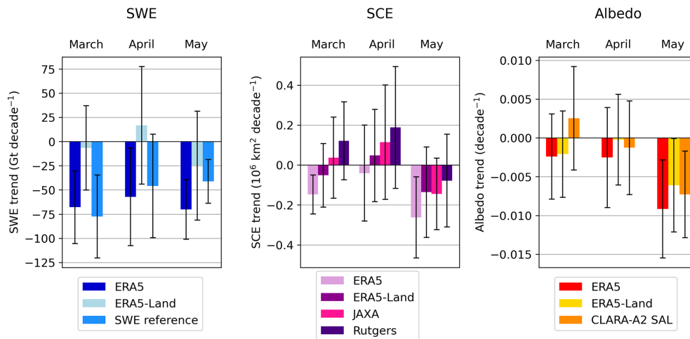
Figure 7. Trends in North America in 1982–2018. The error bars represent the 95 % confidence intervals.
