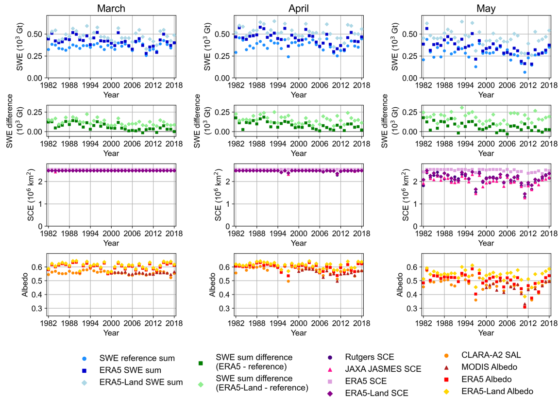
Figure 11. Time series in western Siberia in (left) March, (middle) April, and (right) May for SWE sum (top row), the difference in SWE sum (second row), SCE (third row), and albedo (bottom row). The area is marked in Figs. 9 and 10.
