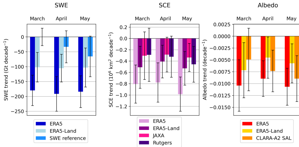
Figure 8. Trends in Eurasia in 1982–2018. The error bars represent the 95 % confidence intervals.
