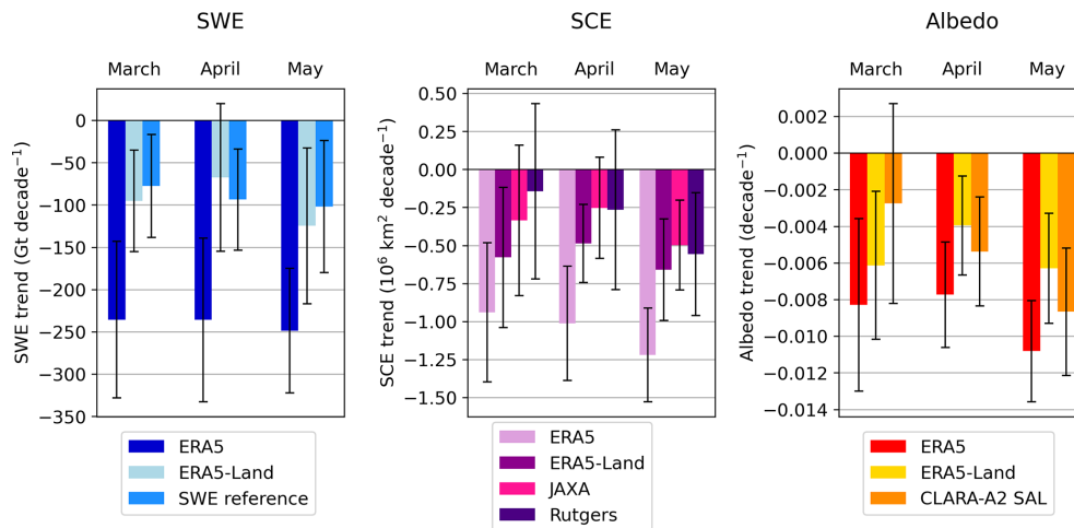
Figure 4. Trends in the Northern Hemisphere in 1982–2018. The error bars represent the 95 % confidence intervals.
