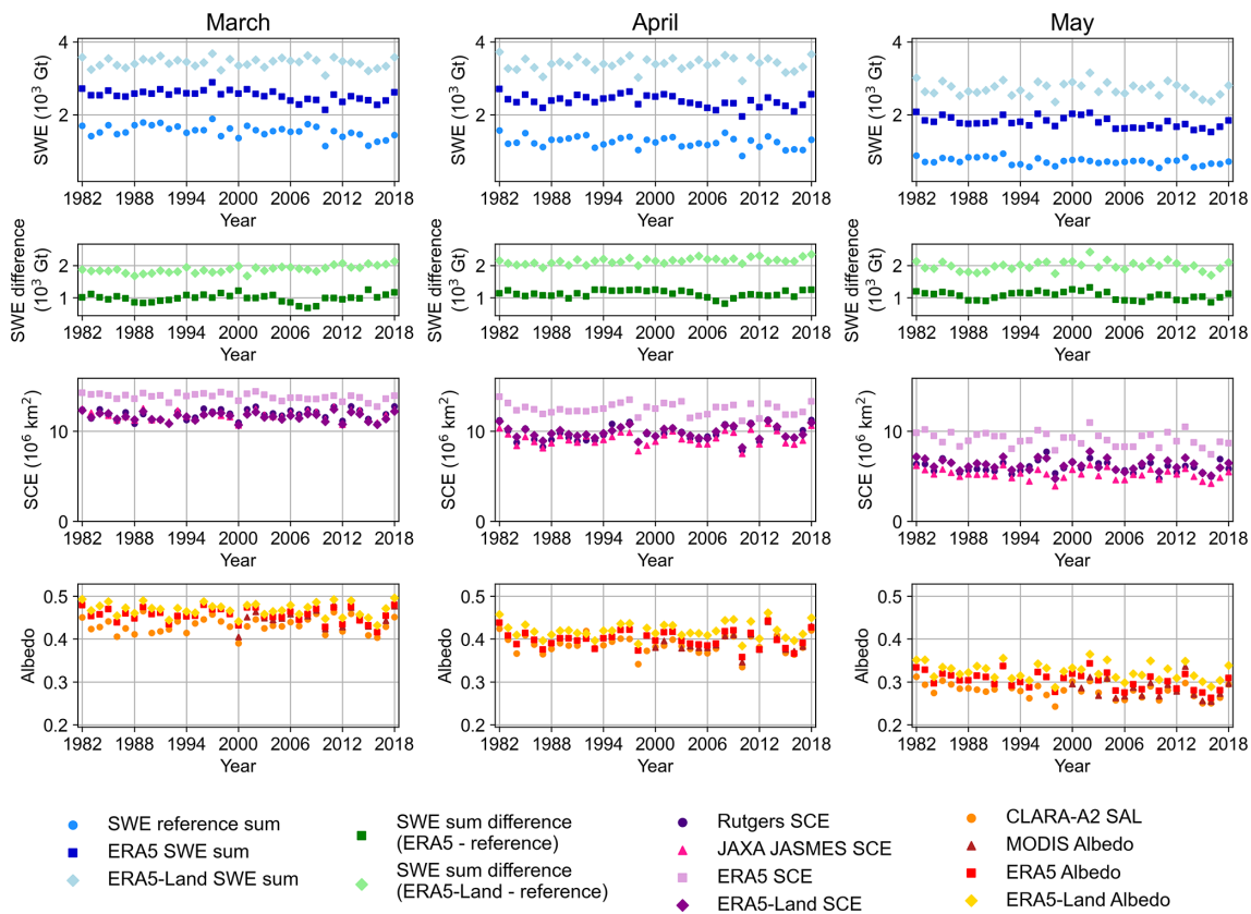
Figure 5. Time series in North America in (left) March, (middle) April, and (right) May for SWE sum (top row), the difference in SWE sum (second row), SCE (third row), and albedo (bottom row).
