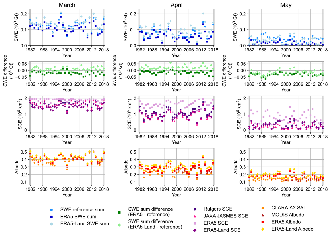
Figure 12. Time series in Canadian Prairies in (left) March, (middle) April, and (right) May for SWE sum (top row), the difference in SWE sum (second row), SCE (third row), and albedo (bottom row). The area is marked in Figs. 9 and 10.
