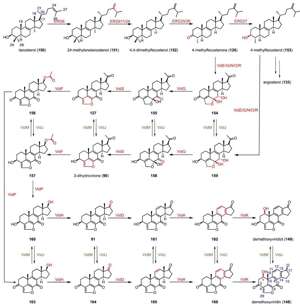
Fig. 28 Biosynthetic pathway of demethoxyviridin and demethoxyviridiol.
