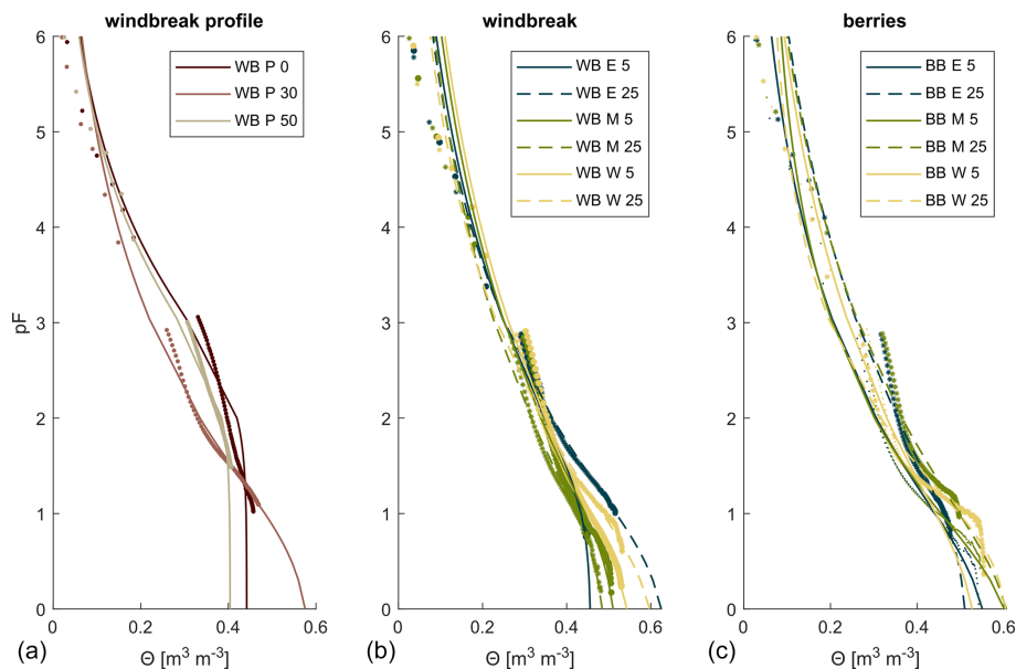
Figure 5. Soil water retention curves of the three profile samples at the windbreak (a, at 0, 0.3 and 0.5 m depth), six samples at three locations at the windbreak (b, at 0.05 and 0.25 m depths) and six samples at three locations in the berries (c, at 0.05 and 0.25 m depths). The dots and stars represent the water tension (pF, the log of the absolute value of the pressure in hPa) and water content measurements, and the lines show the fitted water retention curves after van Genuchten (1980). In panels (b) and (c), dots belong to the 0.05 m depths and stars to the 0.25 m depth.
