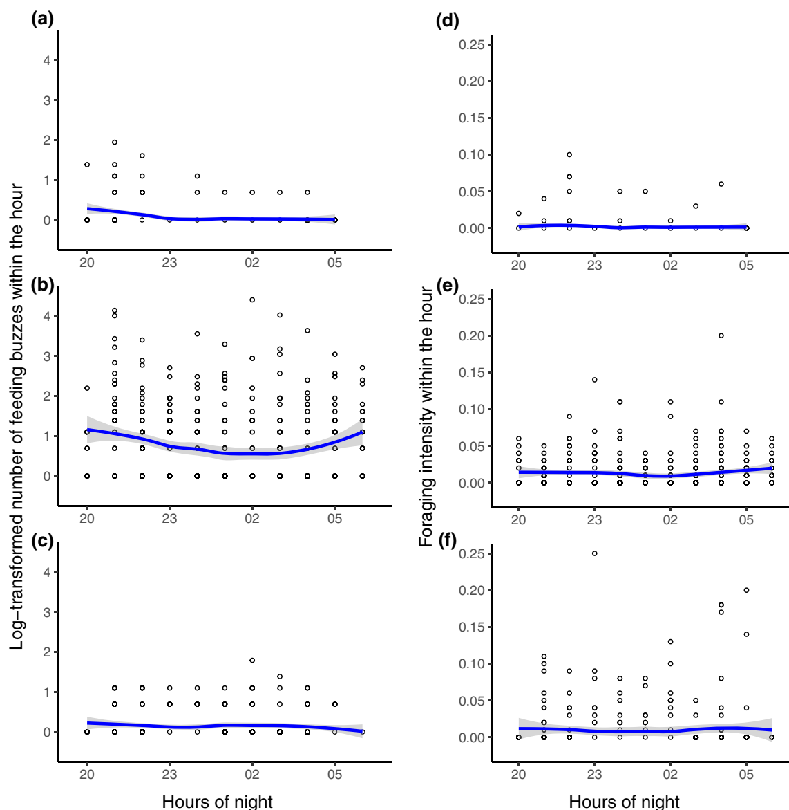
FIGURE 2 (a–c) Log-transformed number of terminal buzzes per hour (1 was added to all zero data points to avoid negative infinite values) and (d–f) the foraging intensity as the proportion of terminal buzzes versus flight activity per hour across the hours of the night for (a and d) open- ( n = 288 ), (b and e) edge- ( n = 494 ), and (c and f) narrow-space foraging bats ( n = 366 ) (Table 1). Note that one data point at foraging intensity of 1 in (f) is not displayed to ensure a better representation of curves and to facilitate comparison among bat guilds. The blue line indicates a loess function (as y \sim x ) that was fitted to the data, while the gray band represents the 95% confidence intervals. Please note that the number of terminal buzzes and the foraging intensity appear pulsed due to hourly aggregation, but were continuous.
