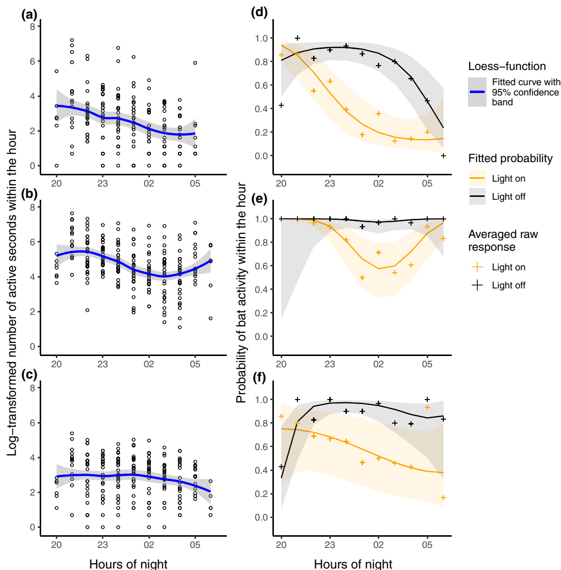
FIGURE 1 (a–c) Echolocation call activity of bats (log-transformed number of active seconds per hour, n_{\text{open-space}} = 205 , n_{\text{edge-space}} = 247 , and n_{\text{narrow-space}} = 229 ) across the night and (d–f) probability of activity (each guild: n = 489 ) in relation to lighting scheme (on/off) for the local functional guilds of open- (a and d), edge- (b and e), and narrow-space foraging bats (c and f) (Table 1). The blue line in (a–c) indicates a loess function (as y \sim x ) that was fitted to the data, while the gray band represents the 95% confidence intervals. Please note that bat activity in (a–c) appears pulsed due to hourly aggregation, but was continuous. Mixed models fitted without the factor “site” were used to achieve a site-independent illustration of the interactive effect between light and time of night (d–f).
